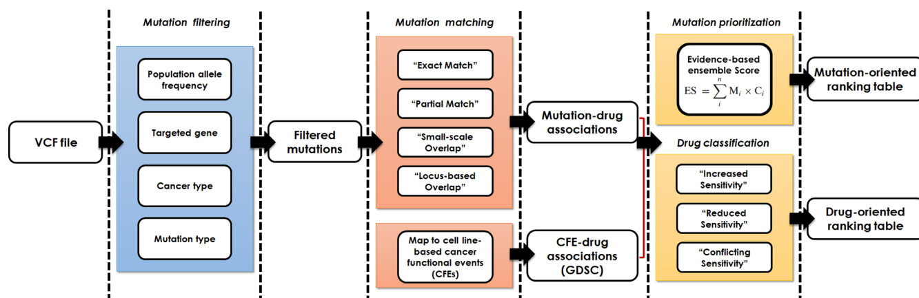
Figure 1. The workflow of mTCTScan (see the description for details of the pipeline).
